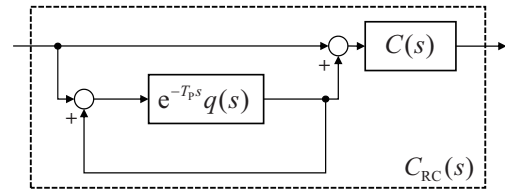
Fig. 6 Repetitive control structure
