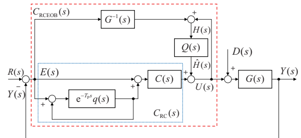
Fig. 3 Structure of the proposed error-based observer improved by a repetitive control strategy (RCEOB)
