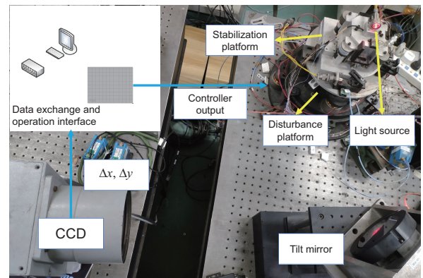
Fig. 17 Composition of the experimental platform
